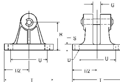
Clevis Bracket
