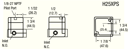
3-Way Pilot
