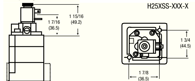
3-Way Single Solenoid
