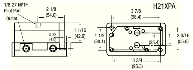
4-Way Pilot
