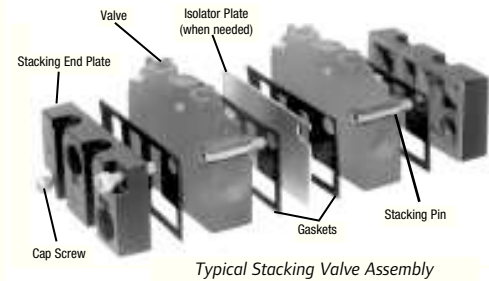
Typical Stacking Valve Assembly
