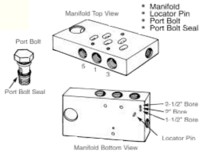
114054 Manifold Kit (1-1/2", 2" and 2-1/2" bores)
