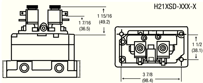
4-Way Double Solenoid
