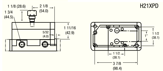
4-Way Pilot Bleed
