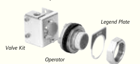
Push Button Assembly
